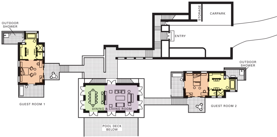
UPPER LEVEL
